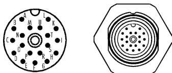
M16 19-pin Male Connector
